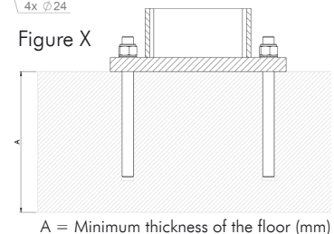
A = Minimum thickness of the floor (mm)
